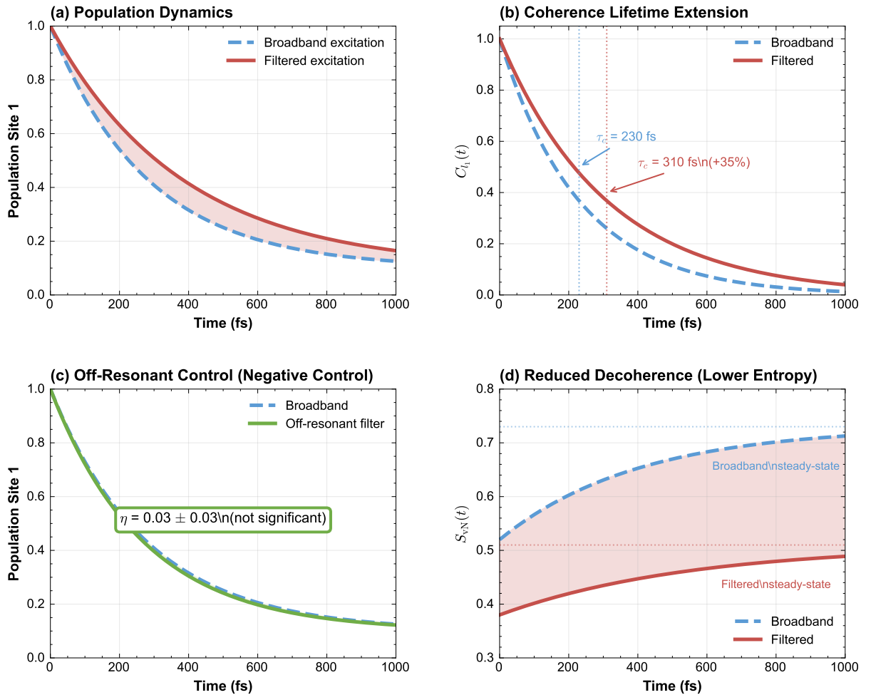
Figure S7: Three-site model dynamics. (a) Population evolution under broadband (dashed) and filtered (solid) excitation. (b) l_1 -norm coherence showing extended lifetime under filtering. (c) Off-resonant filter control showing minimal enhancement. (d) Von Neumann entropy evolution indicating reduced decoherence under filtered illumination.
