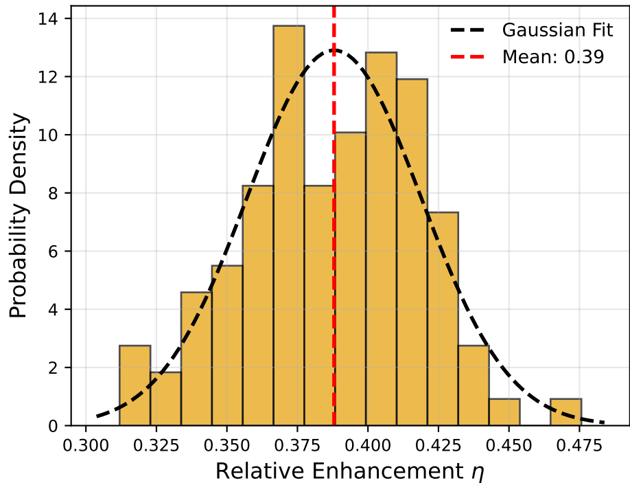
(b) Disorder Robustness ( \sigma = 50 \text{ cm}^{-1} )
