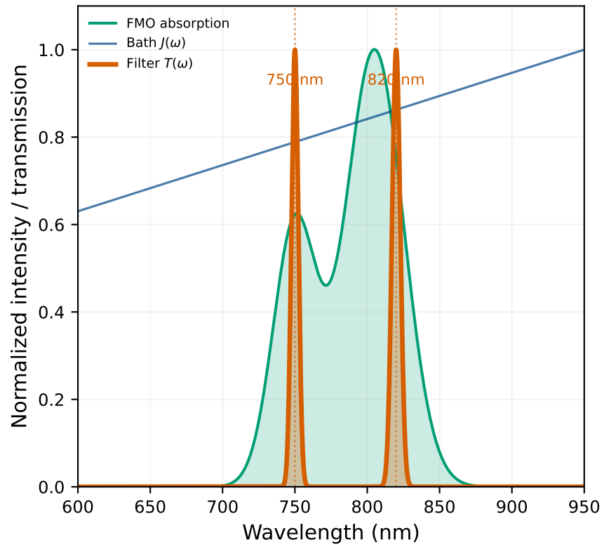
Spectral relationships
