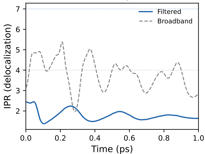
(c) Inverse Participation Ratio
