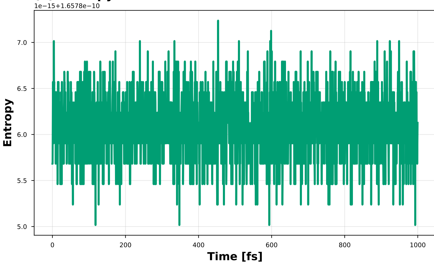
(e) Entropy
