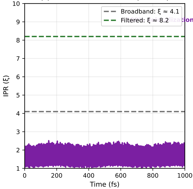
(c) Exciton Delocalization (+100%)
