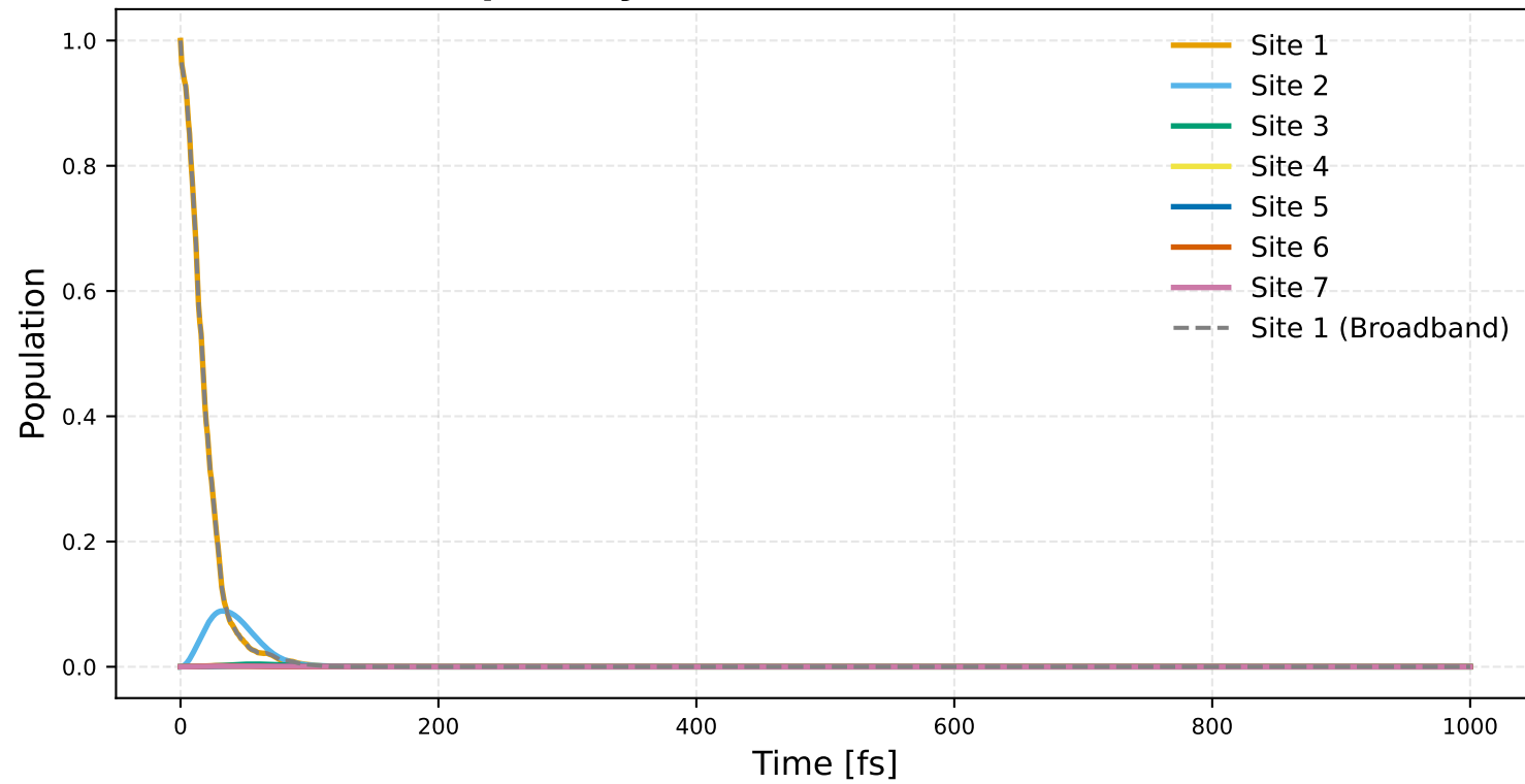
(a) Exciton Transport Dynamics
