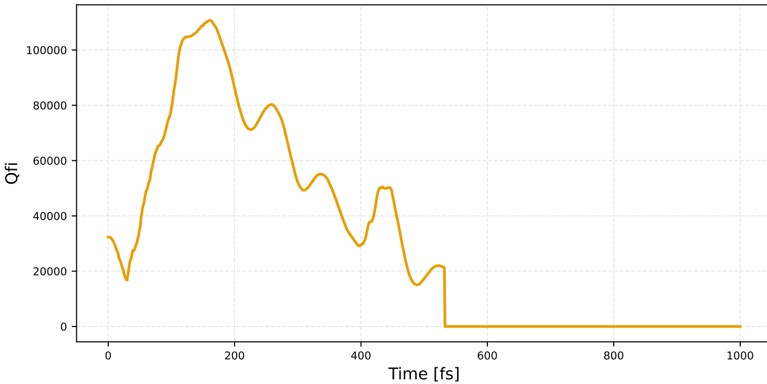
(c) Qfi Evolution
