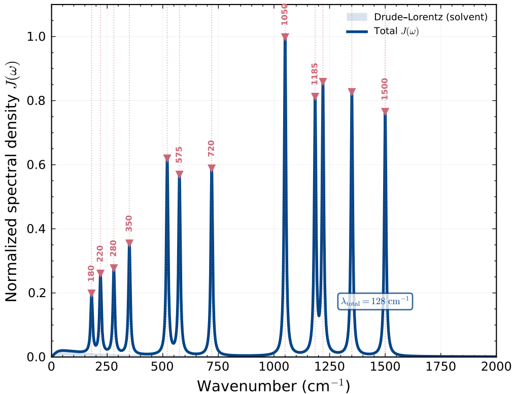
(e) Bath spectral density
