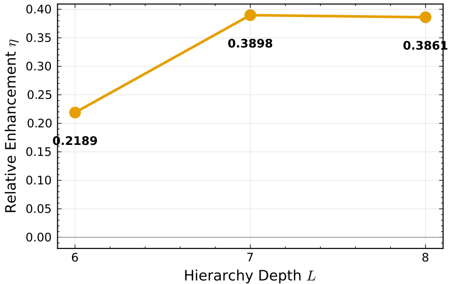
Hierarchy Depth Convergence ( N=5 )
