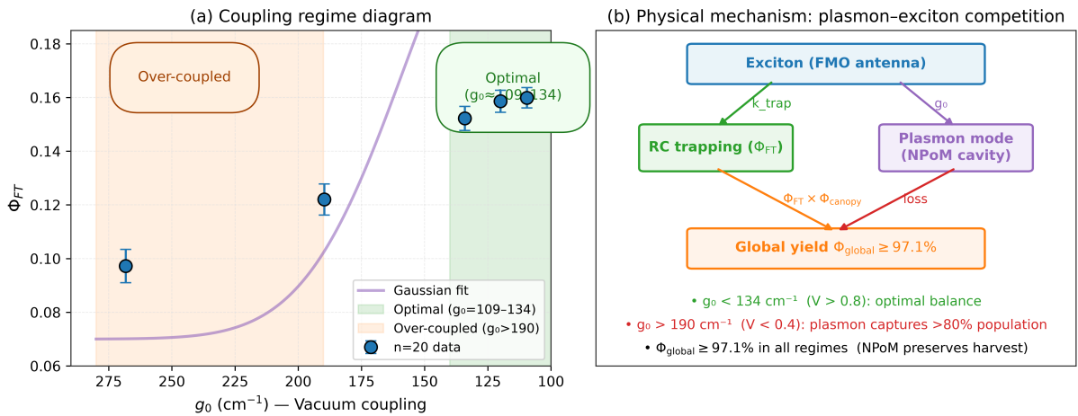
Figure S5: Coupling Regime Diagram. (a) Evolution of \Phi_{\text{FT}} with respect to vacuum coupling g_0 , highlighting the transition from optimal operation to the over-coupled plasmonic trap regime. (b) Schematic representation of the physical mechanism mapping plasmon-exciton competition.
