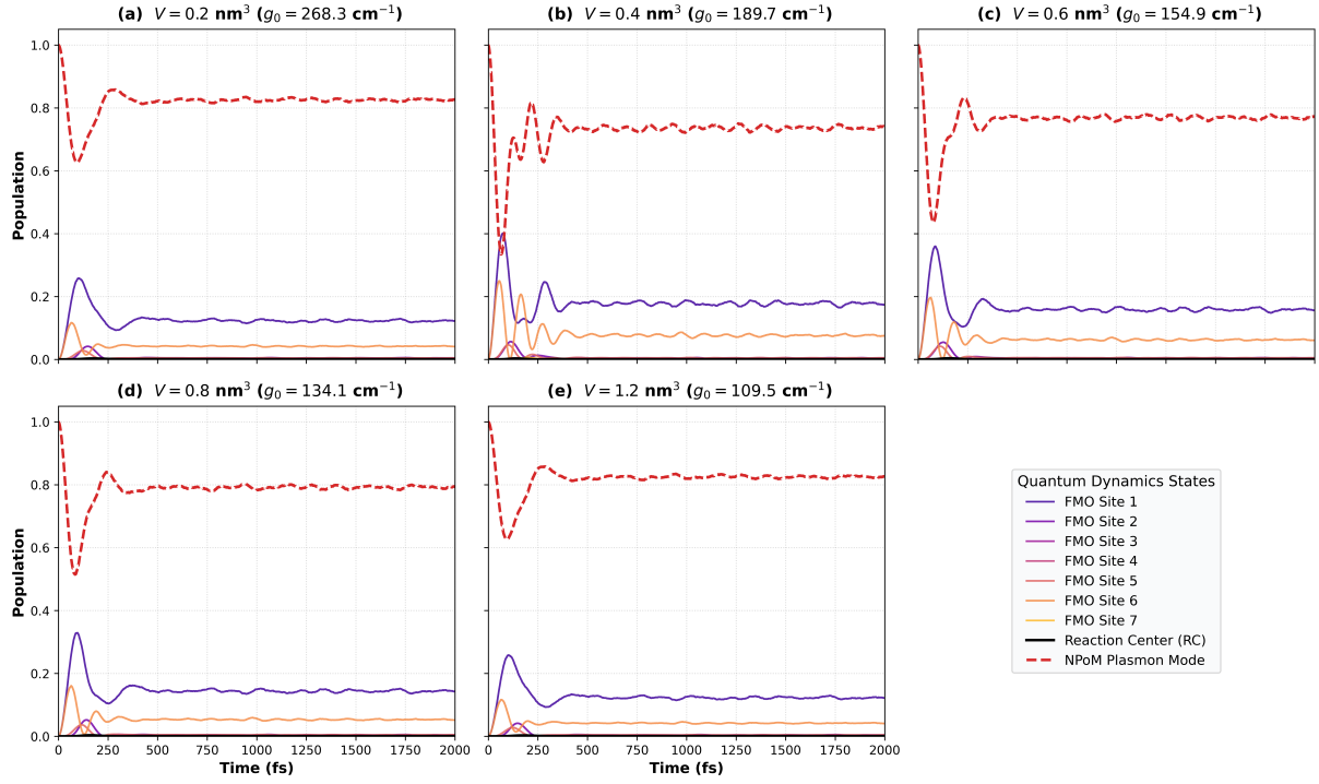
Figure S4: Local exciton-plasmon population dynamics across NPoM mode volumes (2-row layout). Time evolution (0–2000 fs) of the state populations for FMO Sites 1–7 (colored curves), Reaction Center (black curve), and NPoM plasmonic mode (red dashed curve) across mode volumes: (a) V = 0.2 \text{ nm}^3 , (b) V = 0.4 \text{ nm}^3 , (c) V = 0.6 \text{ nm}^3 , (d) V = 0.8 \text{ nm}^3 , and (e) V = 1.2 \text{ nm}^3 . Panel (f) shows the state legend. Arranged in a two-row panel structure for maximum legibility, the dynamics illustrate the severe plasmonic dissipation in the deeply over-coupled limit ( V = 0.2 \text{ nm}^3 ) compared to the smooth, coherent accumulation at the Reaction Center in the optimal domain ( V = 0.8\text{--}1.2 \text{ nm}^3 ).
