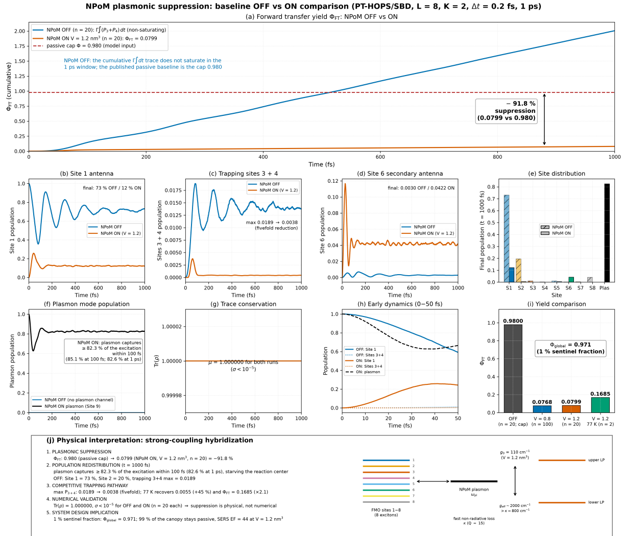
Figure S2: NPoM plasmonic suppression: baseline OFF vs ON comparison. Panel (a): forward transfer yield \Phi_{FT} showing the 91.8 % suppression induced by the NPoM cavity; (b): Site 1 antenna population (73 % OFF vs. 12 % ON); (c): trapping sites 3+4 (fivefold reduction); (d): Site 6 secondary antenna; (e): final site distribution bar chart at t = 1000 fs; (f): plasmon mode population (NPoM ON captures 82 % of total excitation); (g): trace conservation ( \mu = 1.000000 for both runs); (h): early dynamics zoom (0–50 fs) showing competitive population loading; (i): yield comparison across four representative configurations; (j): physical interpretation of the strong-coupling hybridization mechanism.
