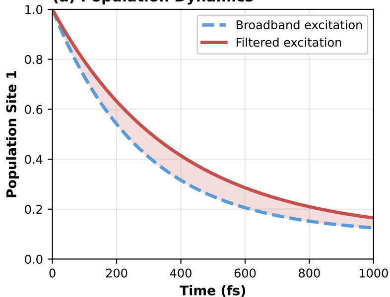
(a) Population Dynamics
