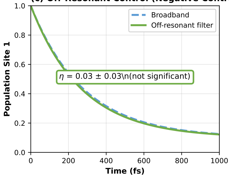
(c) Off-Resonant Control (Negative Control)
