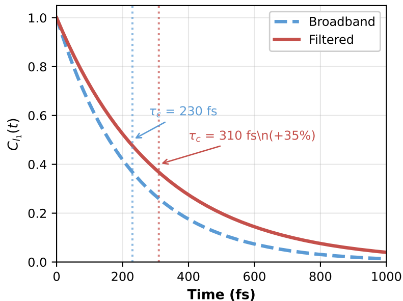
(b) Coherence Lifetime Extension
