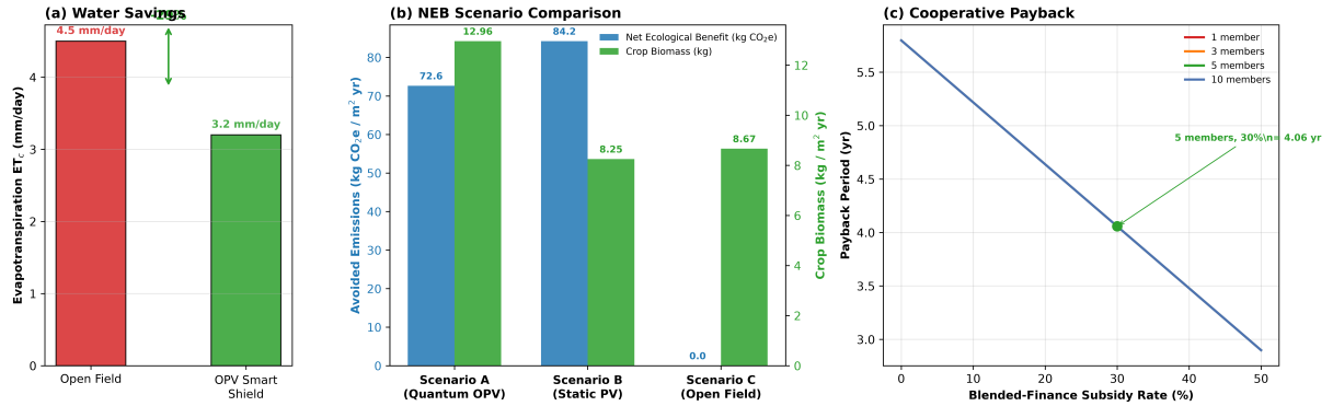
Figure 3: Water–Energy–Food network assessment. (a) FAO-56 evapotranspiration comparison: open field ( ET_c = 4.5 \text{ mm d}^{-1} ) vs. OPV smart shield ( ET_c = 3.2 \text{ mm d}^{-1} ), a 28 % reduction that annualizes to the 474.5 \text{ L m}^{-2} \text{ yr}^{-1} credit of the revenue account. (b) Net Ecological Benefit comparison across three scenarios: Quantum OPV (A), Static shading (B), Open field (C) — the static module buys more carbon but only by suppressing the canopy to 84 % of reference biomass, whereas the quantum shield preserves near-baseline productivity (0.971 global trapping yield, 13.0 with biostimulation). (c) Co-operative payback period as a function of subsidy rate and cooperative size for a 500 \text{ m}^2 floriculture micro-module; the marked point is the 4.32 yr, 5-member, 30 %-subsidy operating point.
