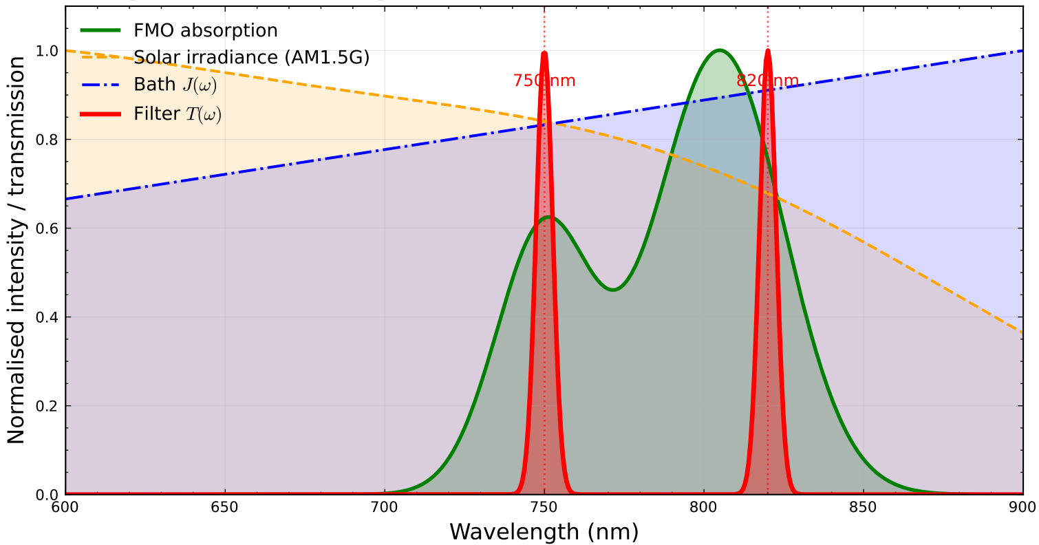
(e) Spectral relationships
