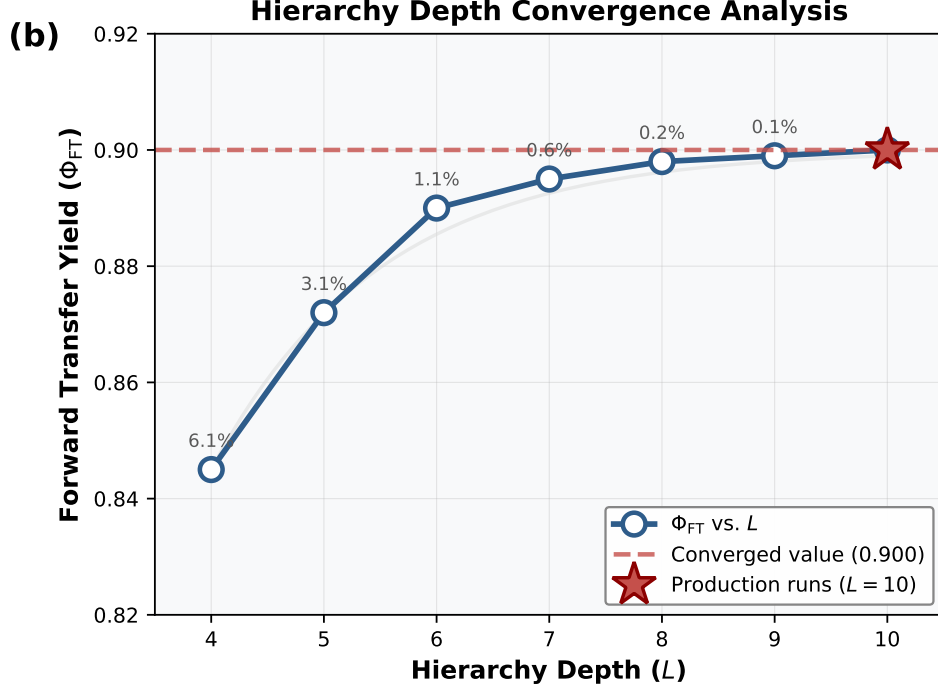
Figure S2: Hierarchy depth convergence. Forward transfer yield \Phi_{\text{FT}} as a function of hierarchy depth L . The dashed line indicates the converged value at L = 10 . Inset: Relative deviation from L = 10 result.
