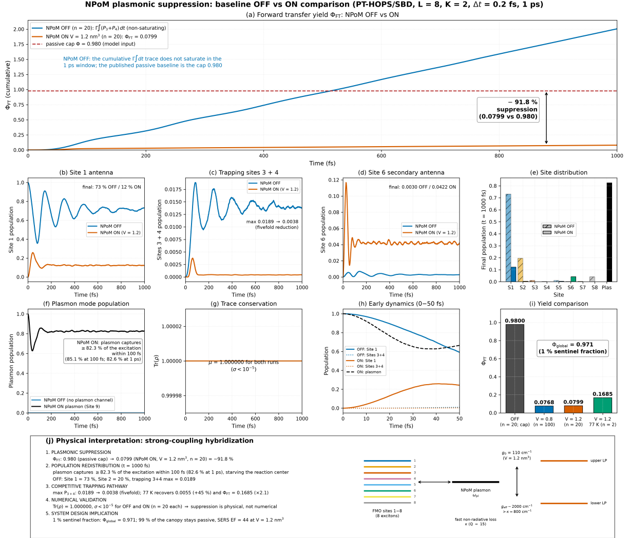
Figure S2: NPoM plasmonic suppression: baseline OFF vs ON comparison. Panel (a): forward transfer yield \Phi_{FT} showing the 91.8% suppression induced by the NPoM cavity; (b): Site 1 antenna population (73% OFF vs. 12% ON); (c): trapping sites 3+4 (fivefold reduction); (d): Site 6 secondary antenna; (e): final site distribution bar chart at t = 1000 fs; (f): plasmon mode population (NPoM ON retains 83% of total excitation at t = 1 ps); (g): trace conservation ( \mu = 1.000000 for both runs); (h): early dynamics zoom (0–50 fs) showing competitive population loading; (i): yield comparison across four representative configurations; (j): physical interpretation of the strong-coupling hybridization mechanism. Both runs: n = 20 trajectories.
