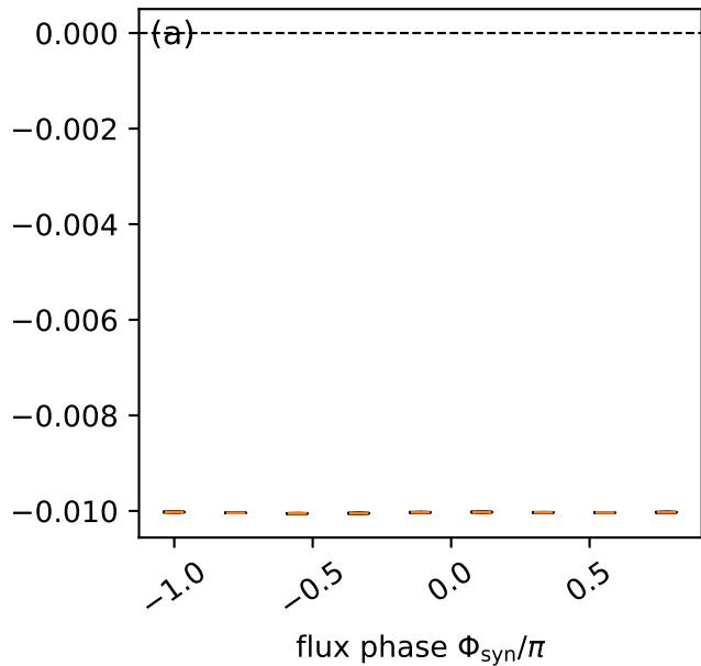
Largest QR exponent \lambda_{\max}
