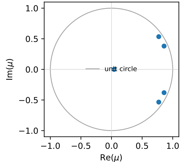
Floquet multipliers
