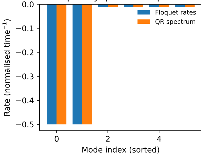
Floquet-Lyapunov comparison
