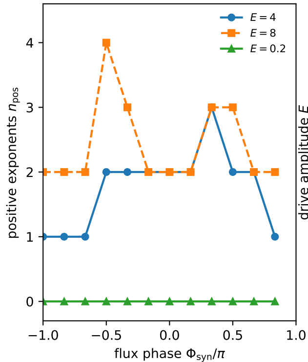
(b) Hyperchaos order vs phase
