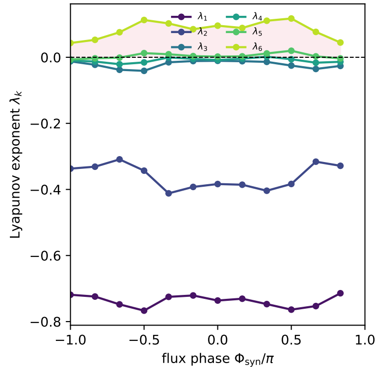
(a) Full spectrum vs phase ( g = 0.3 , E = 4 )
