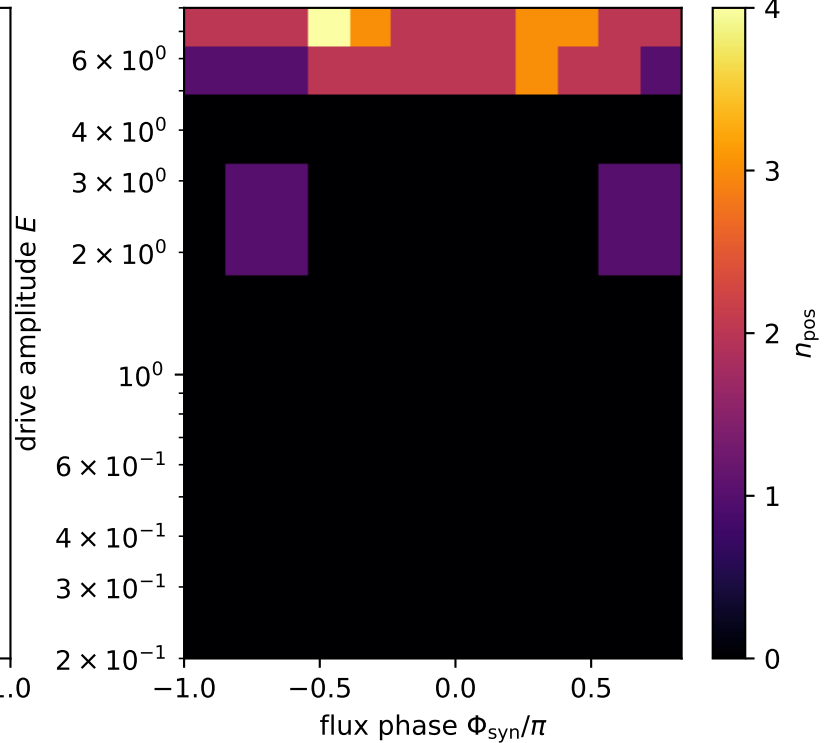
(c) Hyperchaos order n_{\text{pos}}(E, \Phi)
