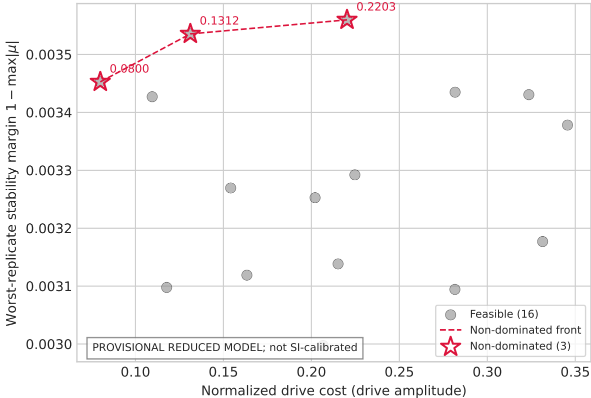
Reduced-model (adiabatic) Pareto front: stability margin vs drive cost
