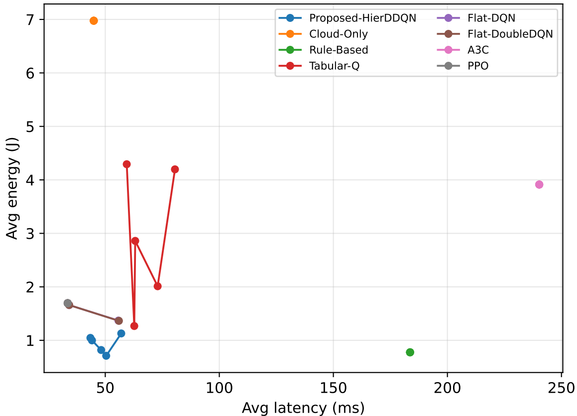
Latency-energy Pareto front (weight grid)
