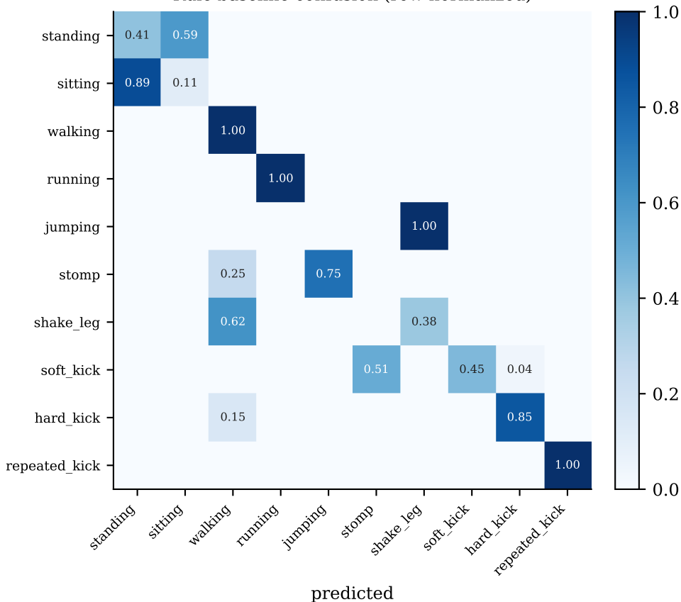
Rule baseline confusion (row normalized)
