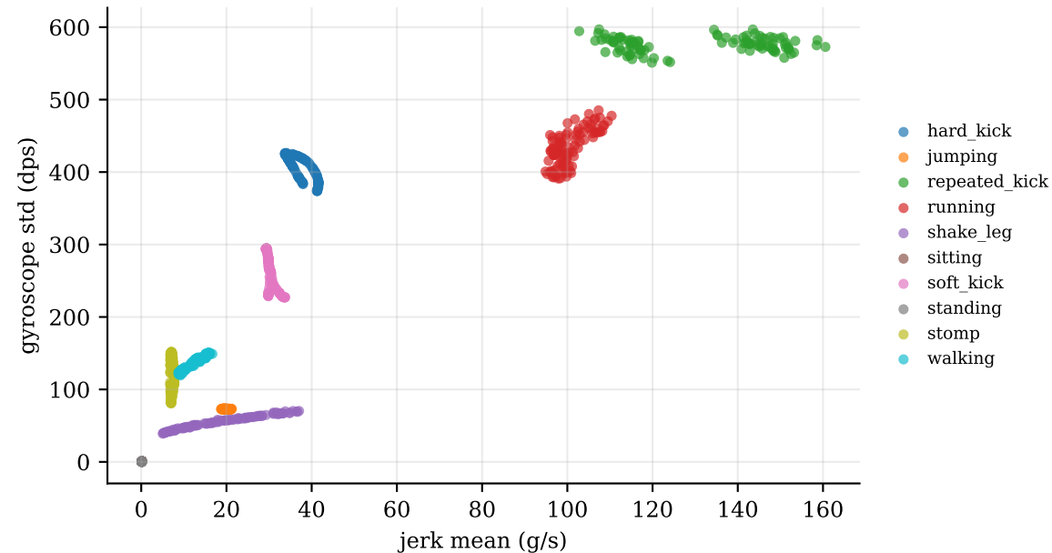
Two feature view of class clusters
