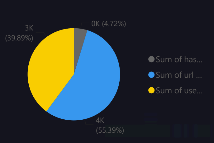
Interaction Distribution
