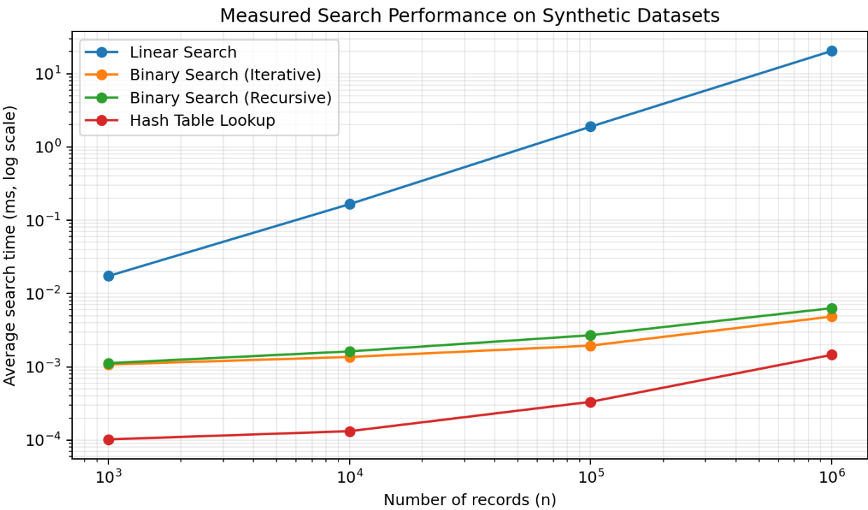
Figure 1. Experimental search-time comparison (logarithmic axes).
