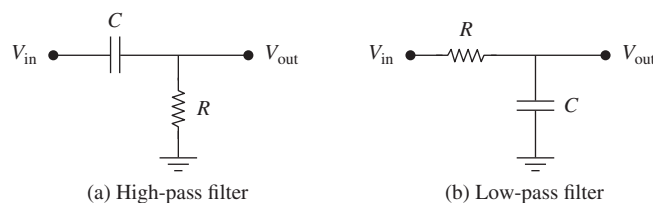
Figure 7.1 Example circuit diagrams for high- and low-pass filters.
