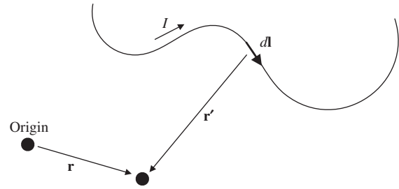
Figure 2.12 Calculating magnetic field from the Biot–Savart law.
