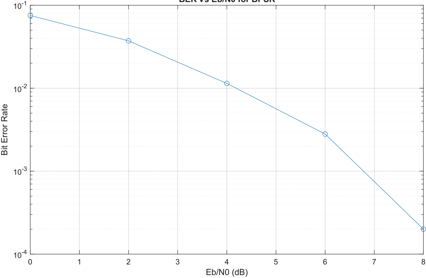
BER vs Eb/N0 for BPSK
