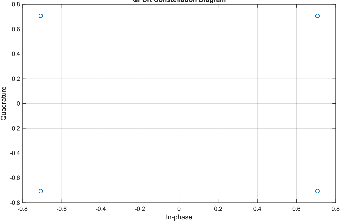
QPSK Constellation Diagram
