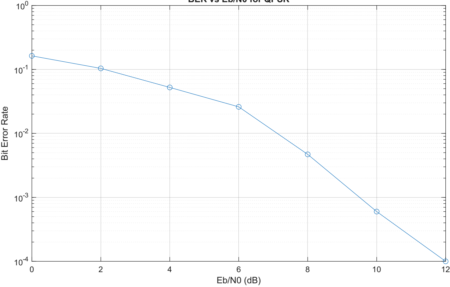
BER vs Eb/N0 for QPSK
