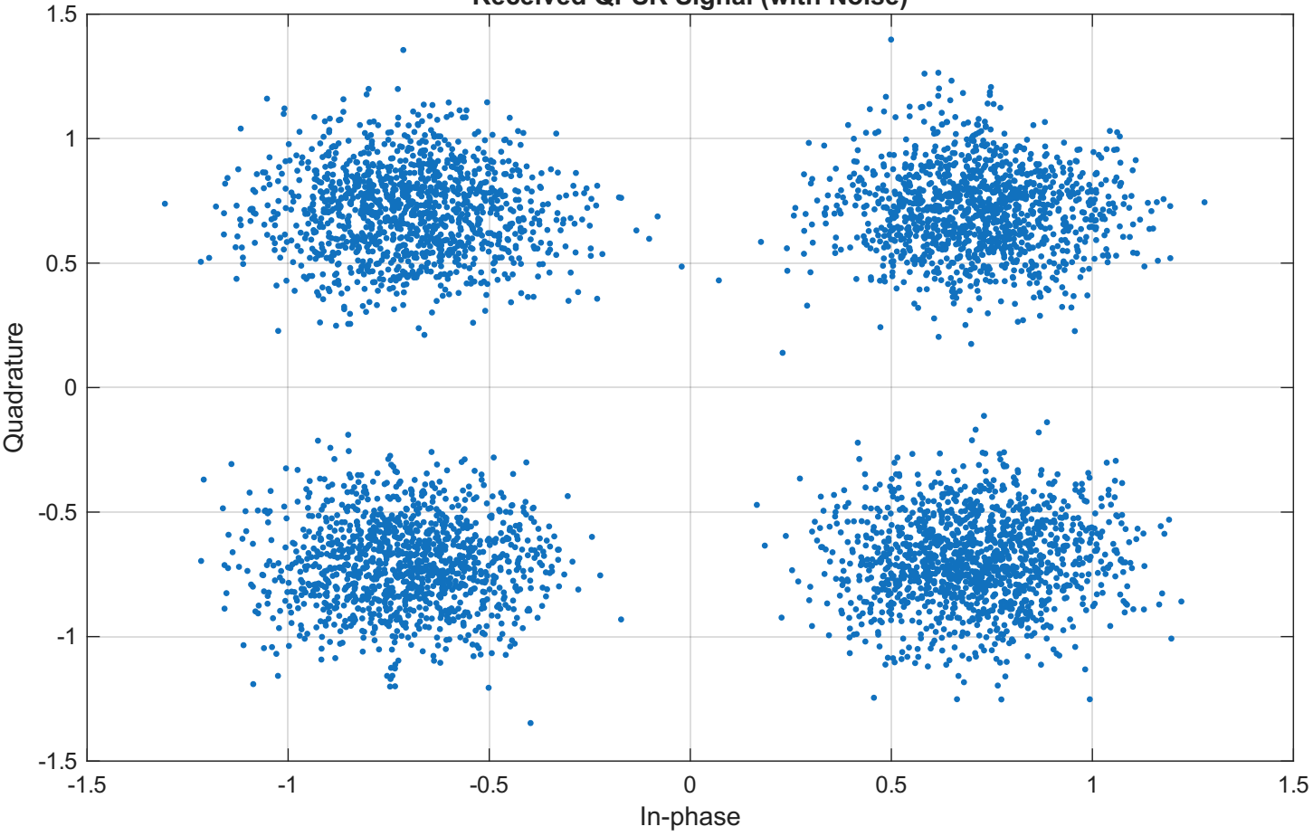
Received QPSK Signal (with Noise)
