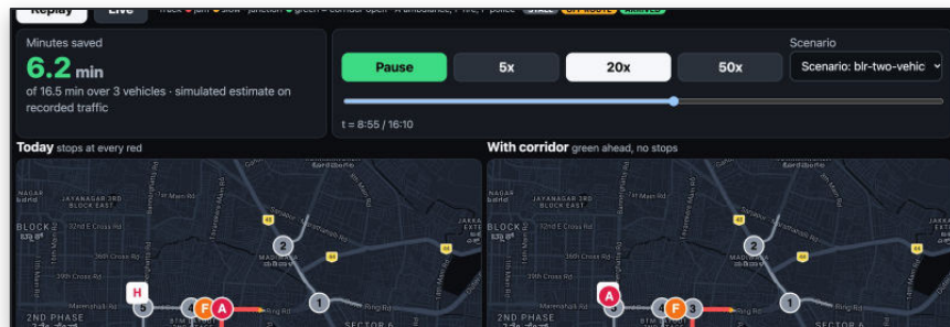
Replay simulator
