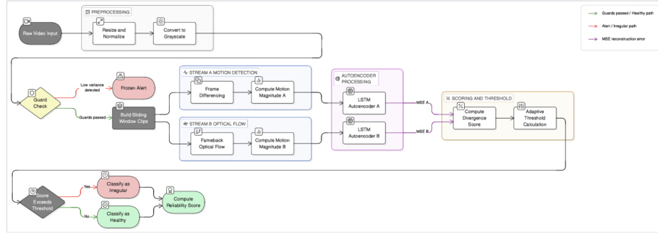
Fig. 1: Proposed Adaptive Dual-Stream LSTM-AE pipeline. The guard layer filters trivial failures before dual-stream LSTM-AE processing and divergence-based scoring.
