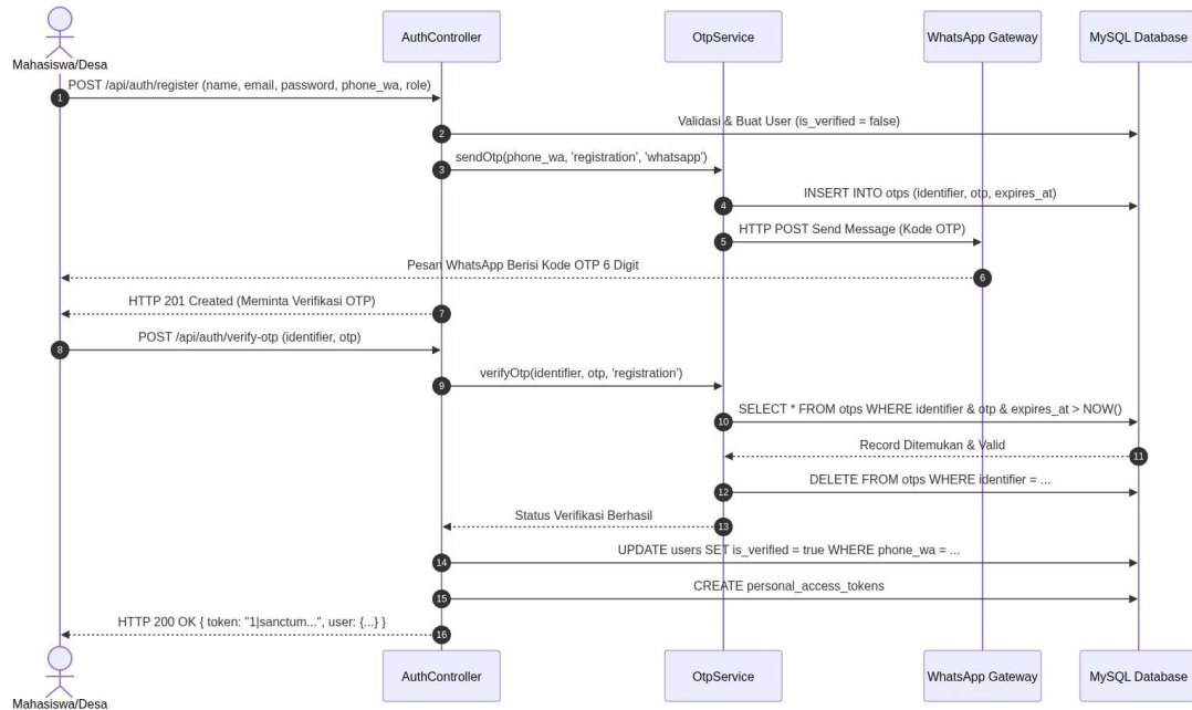
Gambar 5.5: Sequence Diagram Alur Autentikasi & OTP Multi-Channel
