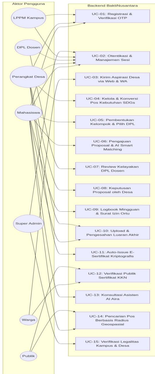
Gambar 5.1: Use Case Diagram Sistem Backend BaktiNusantara
