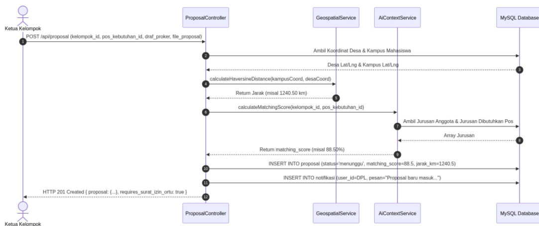
Gambar 5.6: Sequence Diagram Pengajuan Proposal & Perhitungan Haversine
