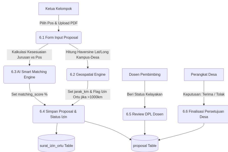
Gambar 3.4: DFD Level 2 - Proses 6.0 (Proposal, AI Matching & Geospasial)
