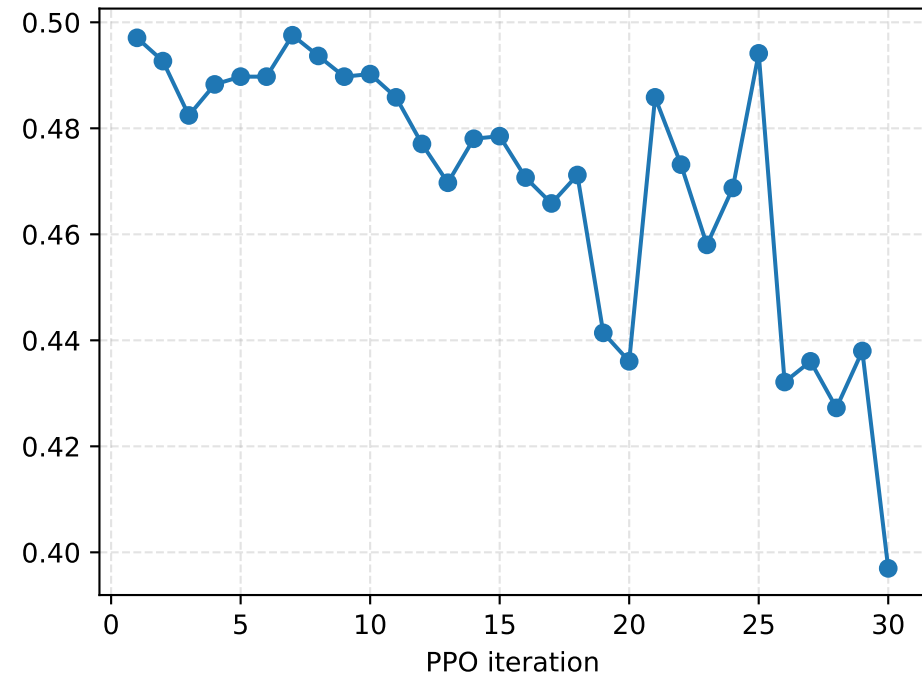
Keep ratio
