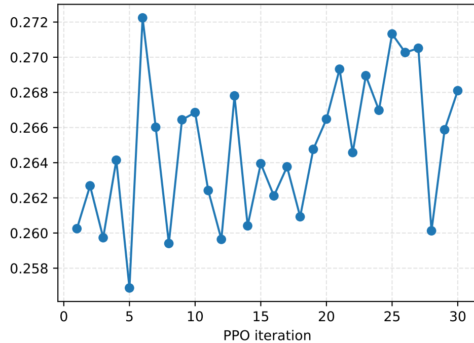
Episode reward
