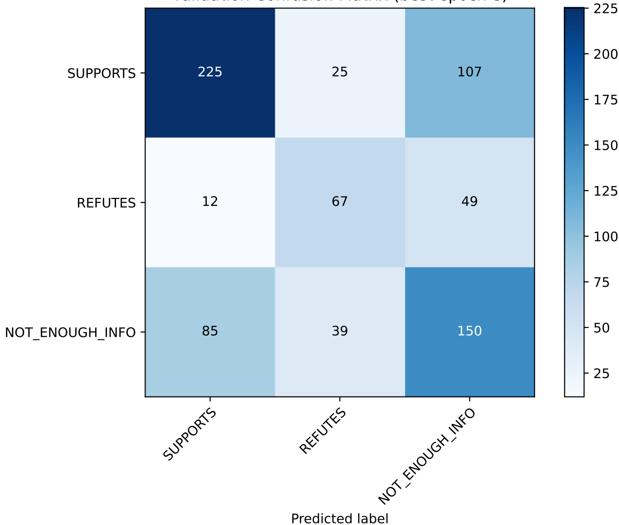
Validation Confusion Matrix (best epoch 8)
