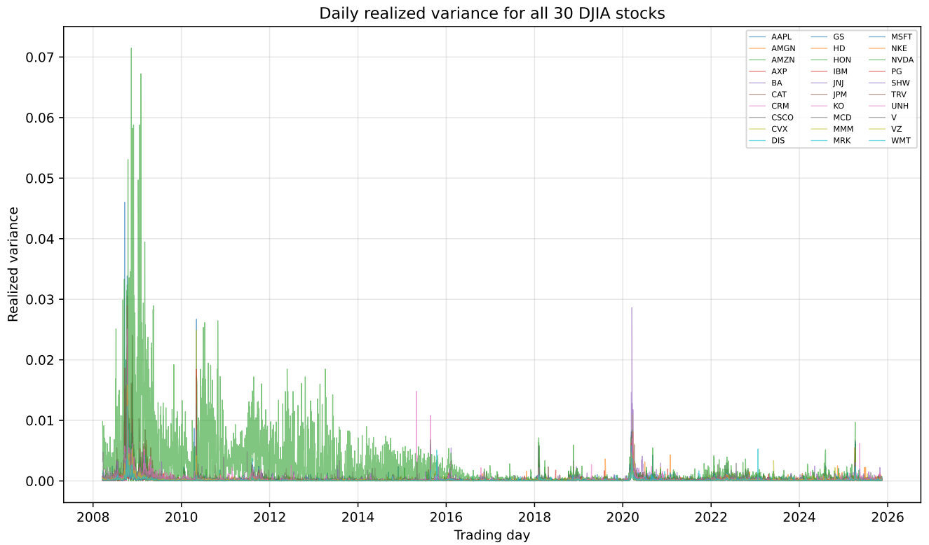
Figure 2: Daily realized variances for the 30 DJIA stocks.
