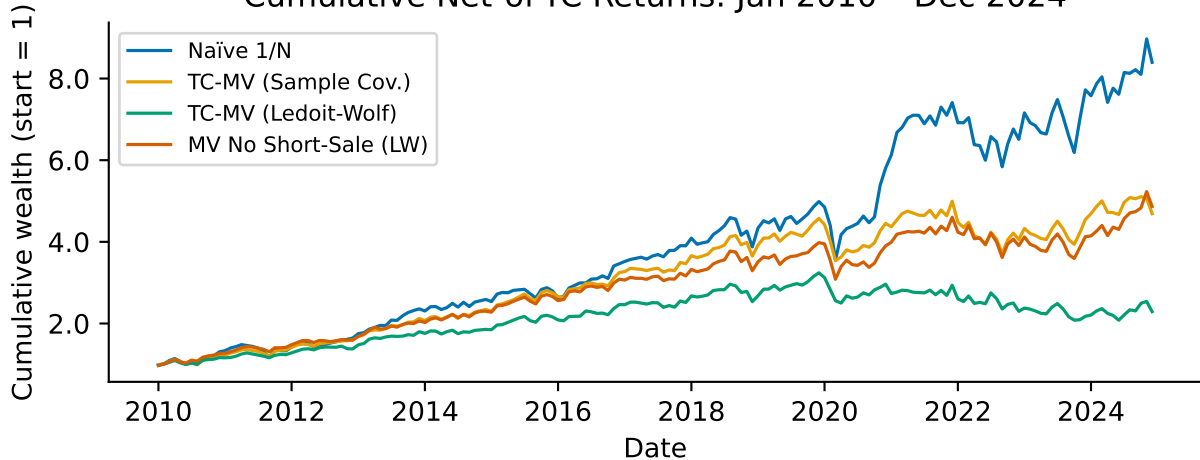
Cumulative Net-of-TC Returns: Jan 2010 – Dec 2024
