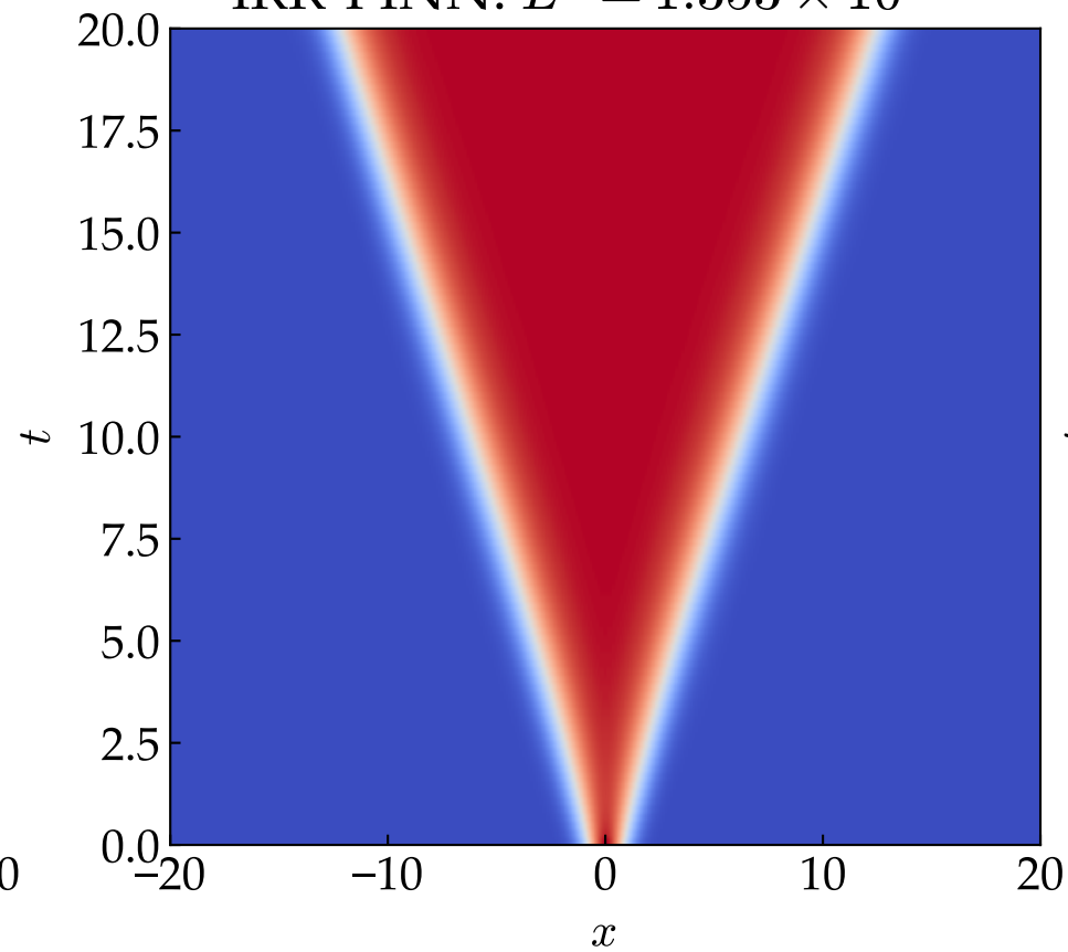
IRR-PINN: L^2 = 1.353 \times 10^{-02}
