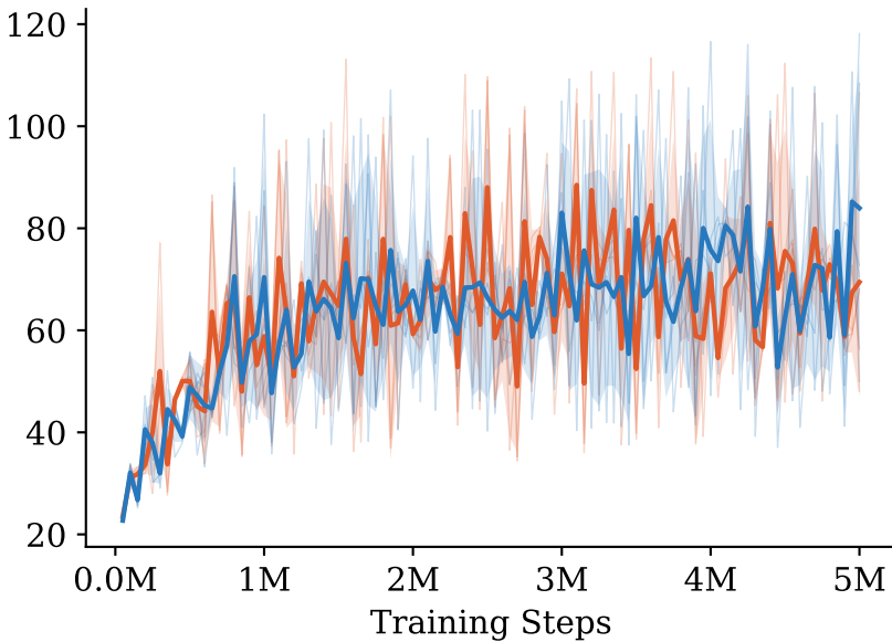
Episode Length (steps survived)
