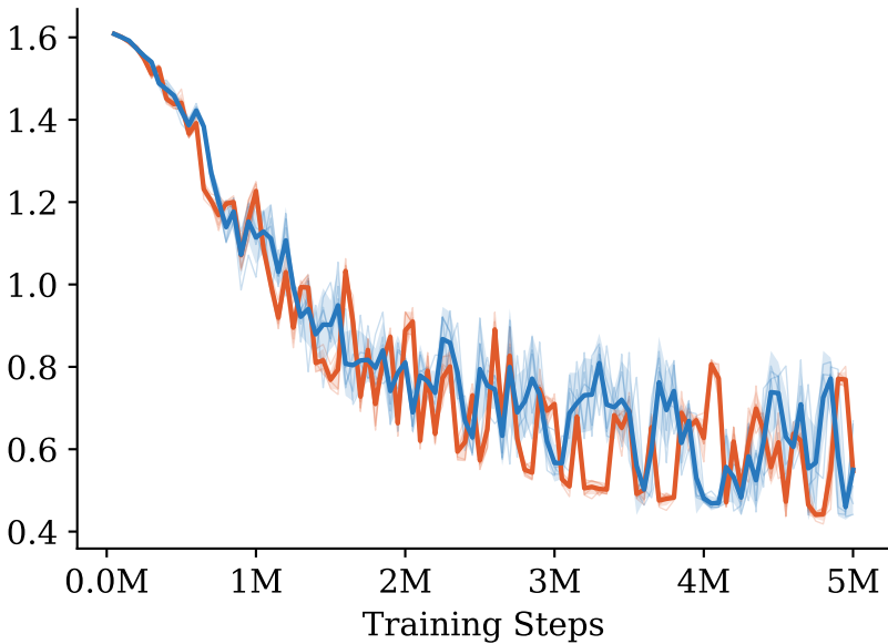
Policy Entropy
