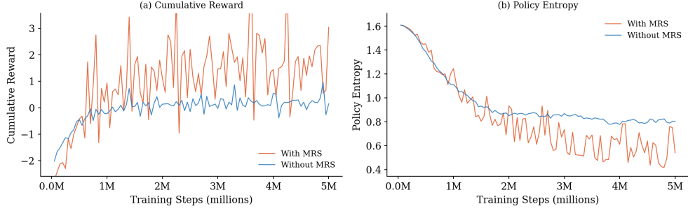
Fig. 3: Ablation of the MRS observation channel: training diagnostics with the market-information channel present (“With MRS”) versus removed (“Without MRS”). (a) Cumulative reward and (b) policy entropy over 5 \times 10^6 training steps. Both policies are trained under identical architecture, hyperparameters, and random seed; they differ only in whether the MRS channel is present in the observation.
