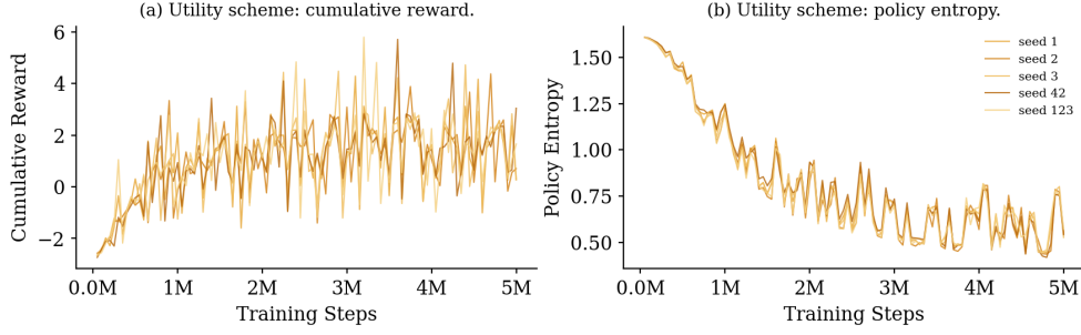
Fig. 2: Learning diagnostics across five independent training seeds ( \{1, 2, 3, 42, 123\} ). (a) Cumulative reward and (b) policy entropy over 5 \times 10^6 training steps. All seeds follow closely consistent convergence trajectories, indicating that training is reproducible and not dependent on a fortunate seed.
