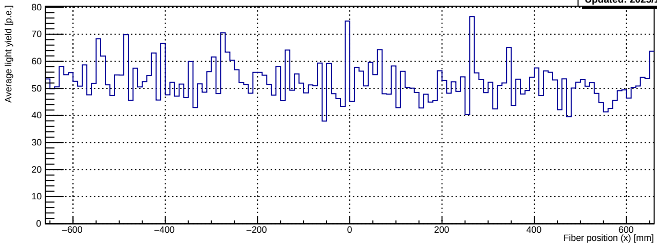
Average light yield vs fiber position (x)
