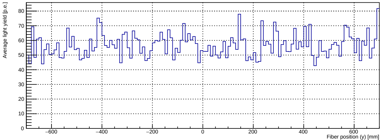
Average light yield vs fiber position (y)
