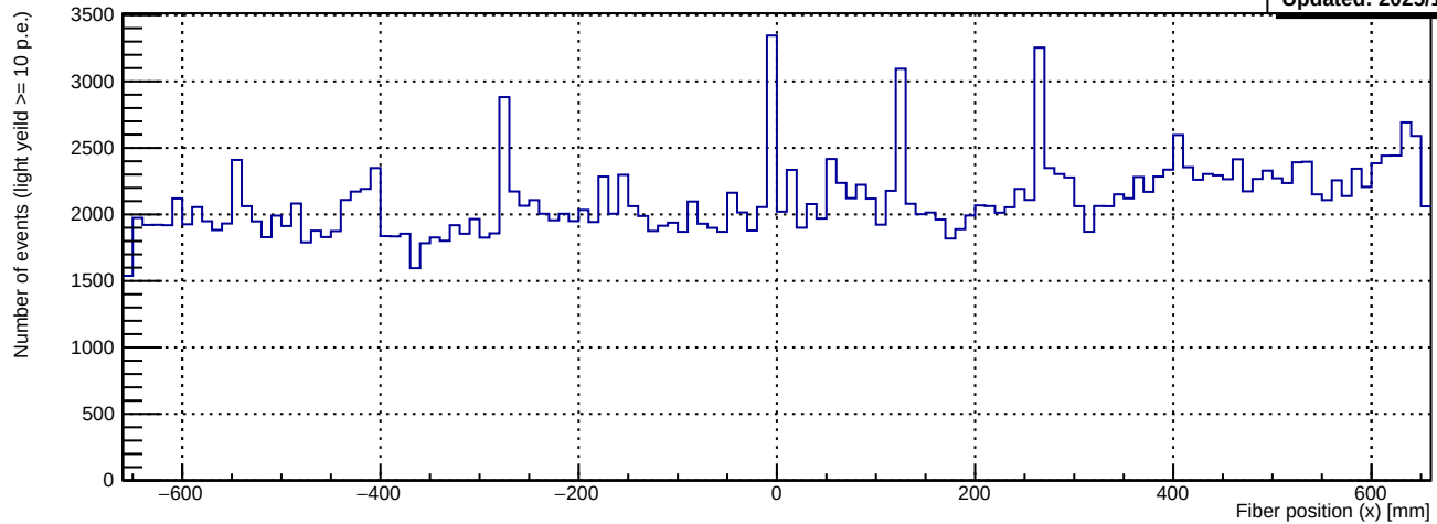
Number of events with light yield \geq 10 p.e. vs fiber position (x)
