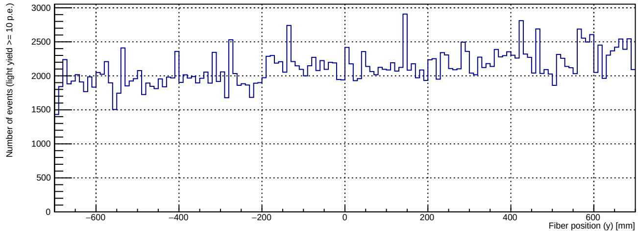
Number of events with light yield \geq 10 p.e. vs fiber position (y)
