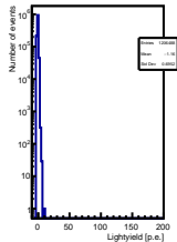
RAYRAW99 ch27 (cable 281)
