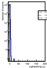
RAYRAWW10 ch20 (cable 300)
