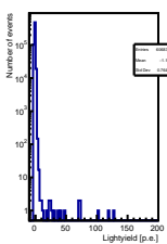
RAYRAW10 ch08 (cable 292)
