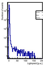
RAYRAWW6 ch12 (cable 136)
