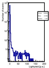
RAYRAWW6 ch17 (cable 201)
