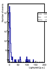
RAYRAW10 ch27 (cable 305)
