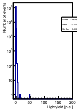
RAYRAWW10 ch11 (cable 295)
