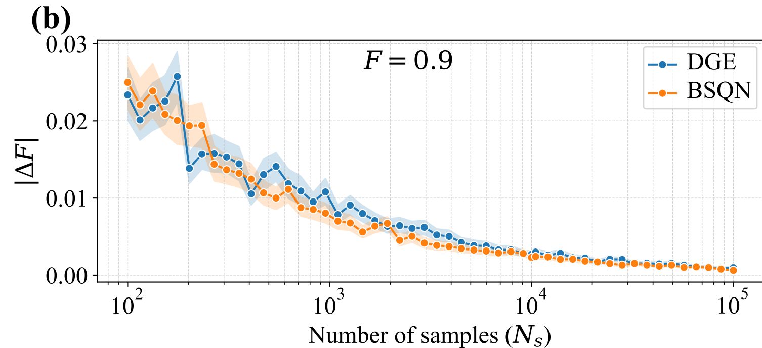
Performance comparison between BSQN and DGE on complete graph ( n = 8 )
