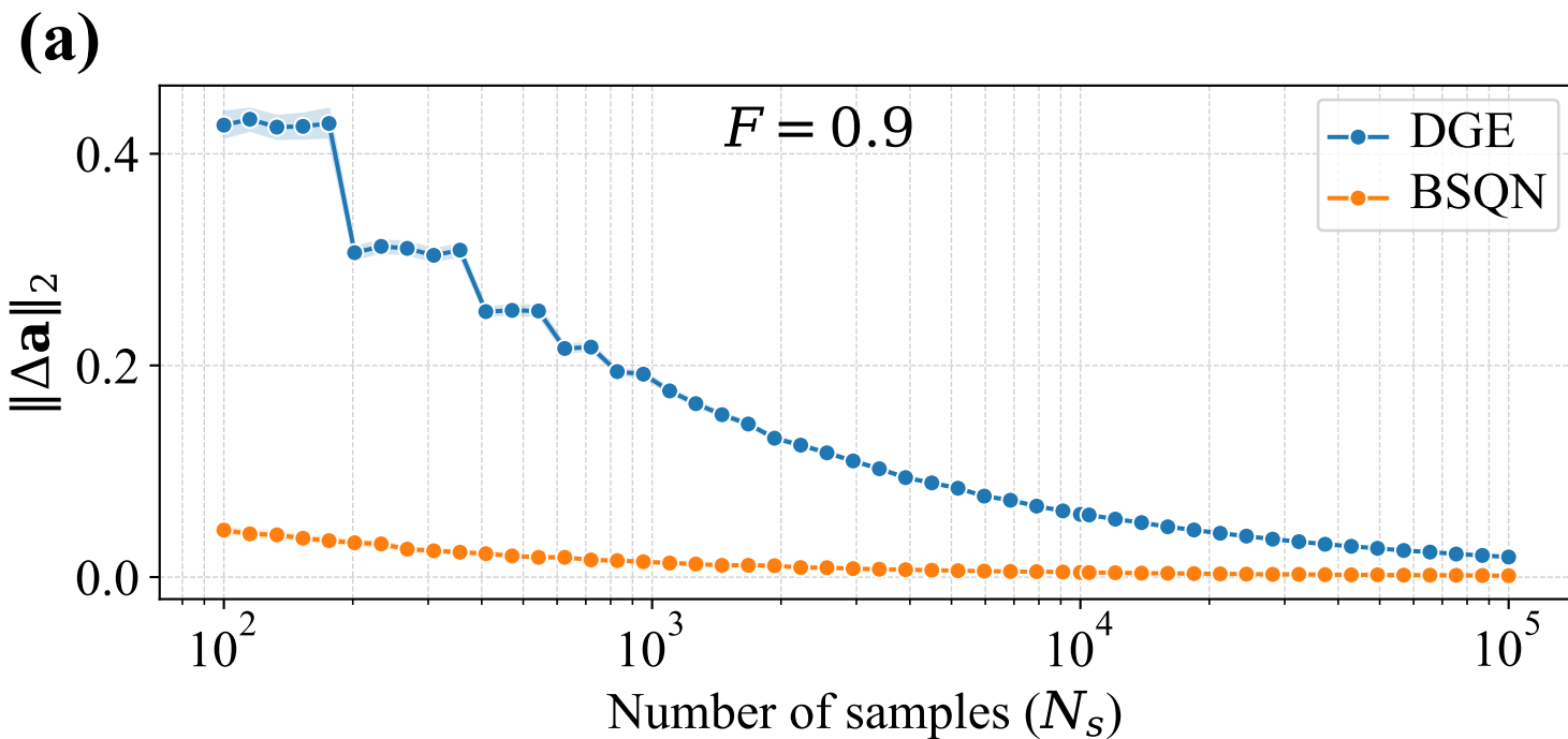
Performance comparison between BSQN and DGE on complete graph ( n = 8 )
