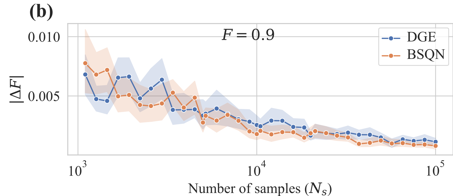
Performance comparison between BSQN and DGE on complete graph ( n = 12 )
