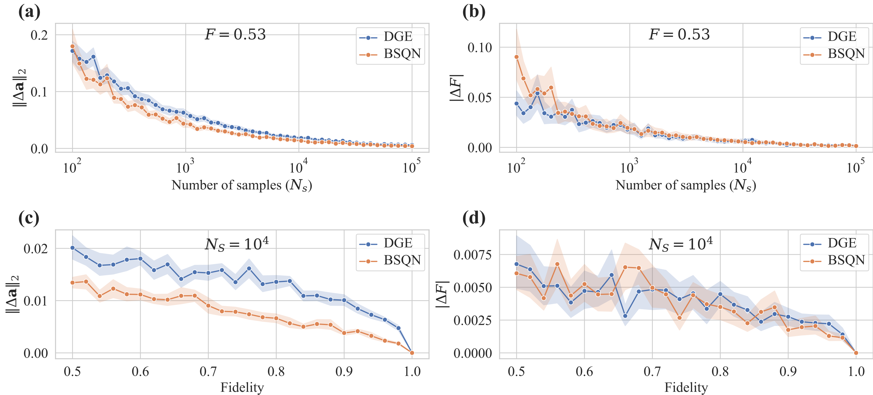
Performance comparison between BSQN and DGE on complete graph ( n = 3 )
