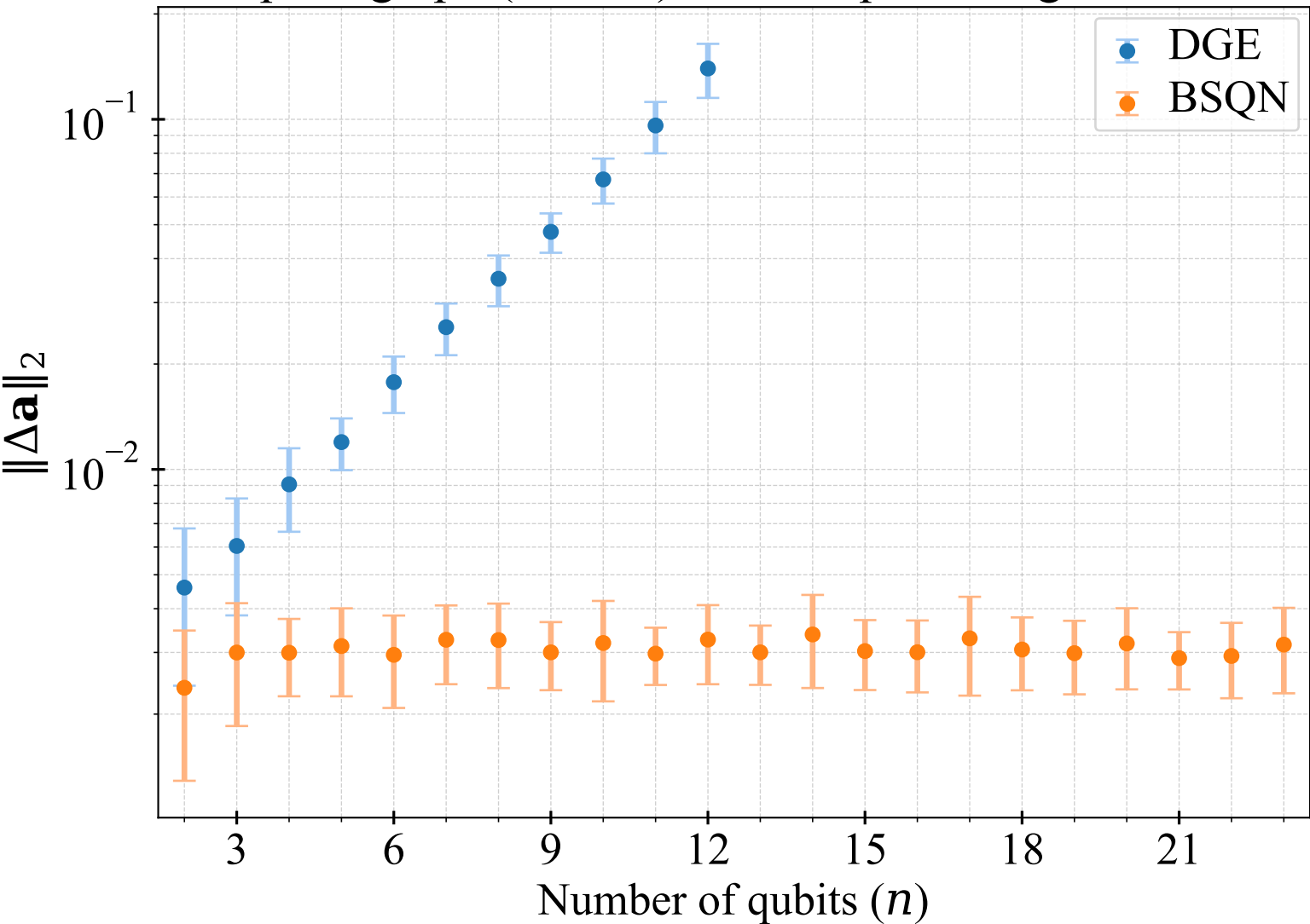
Complete graph ( F = 0.9 ) under depolarizing noise ( \mathcal{N}_1 )
