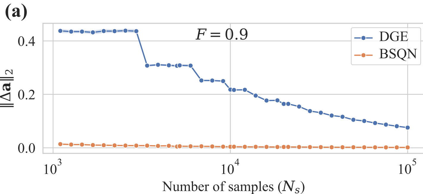
Performance comparison between BSQN and DGE on complete graph ( n = 12 )
