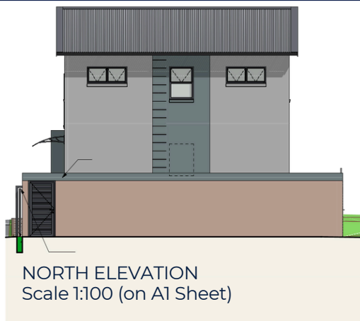
North Elevation
