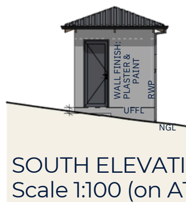
South Elevation
