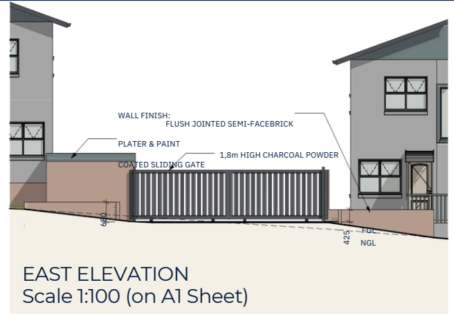
East Elevation
