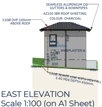
East Elevation
