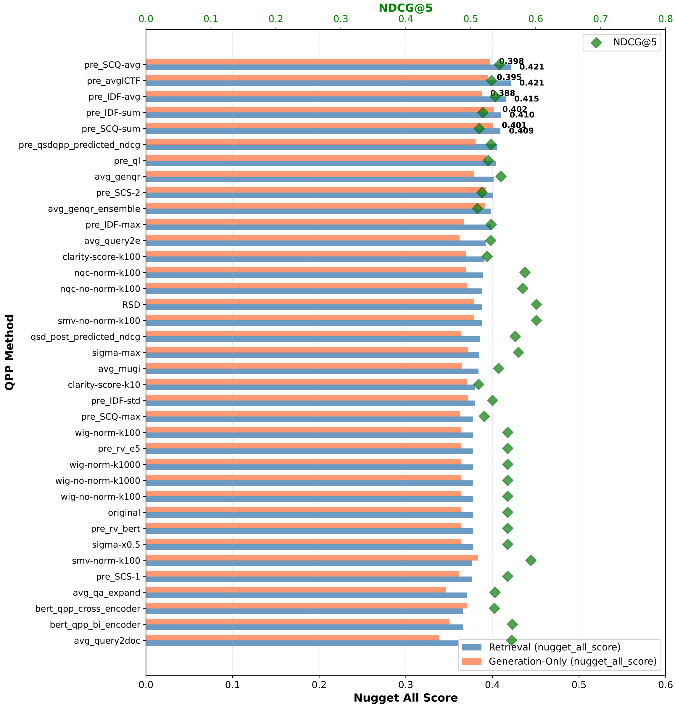
Dense Retriever (Cohere)
