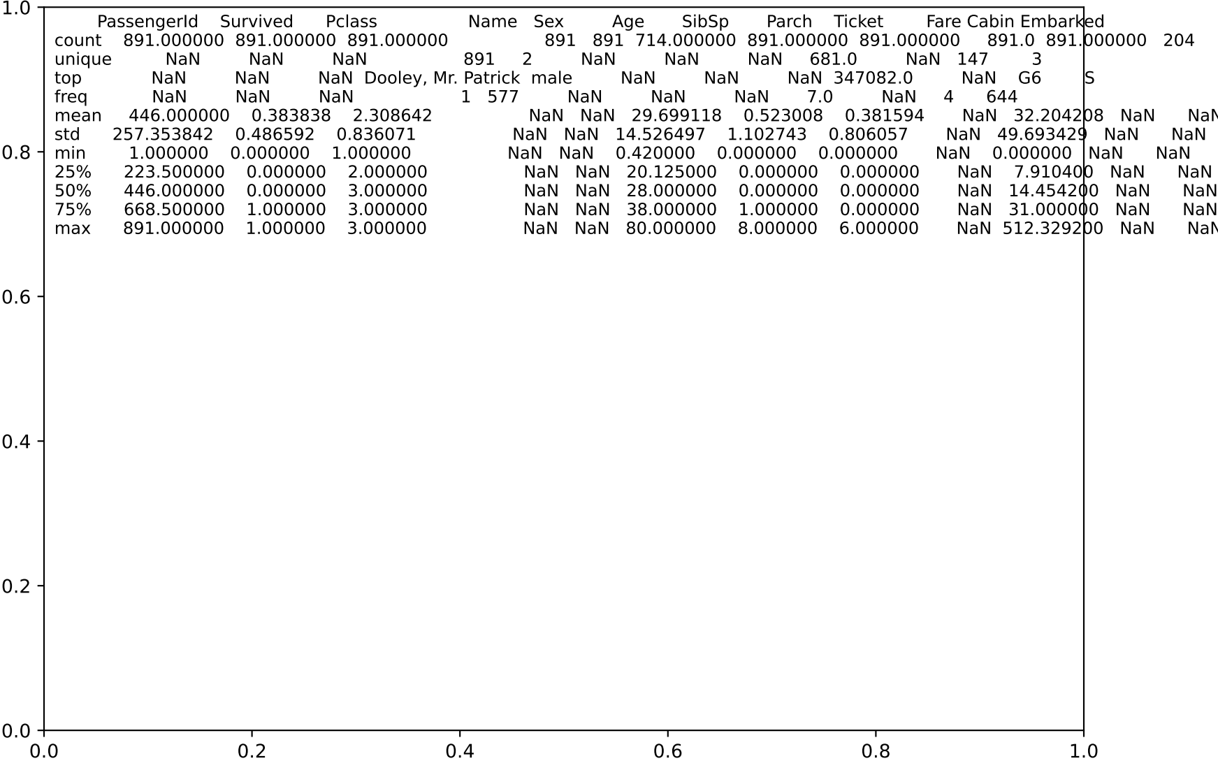
Describe Statistics
