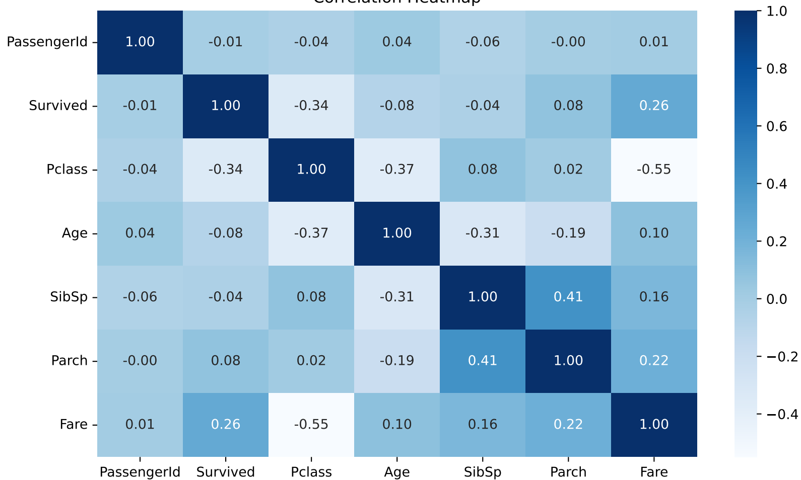
Correlation Heatmap
