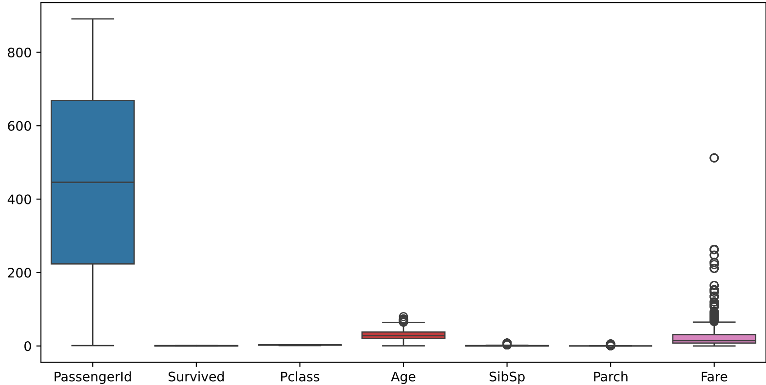
Boxplot - Numerical Columns
