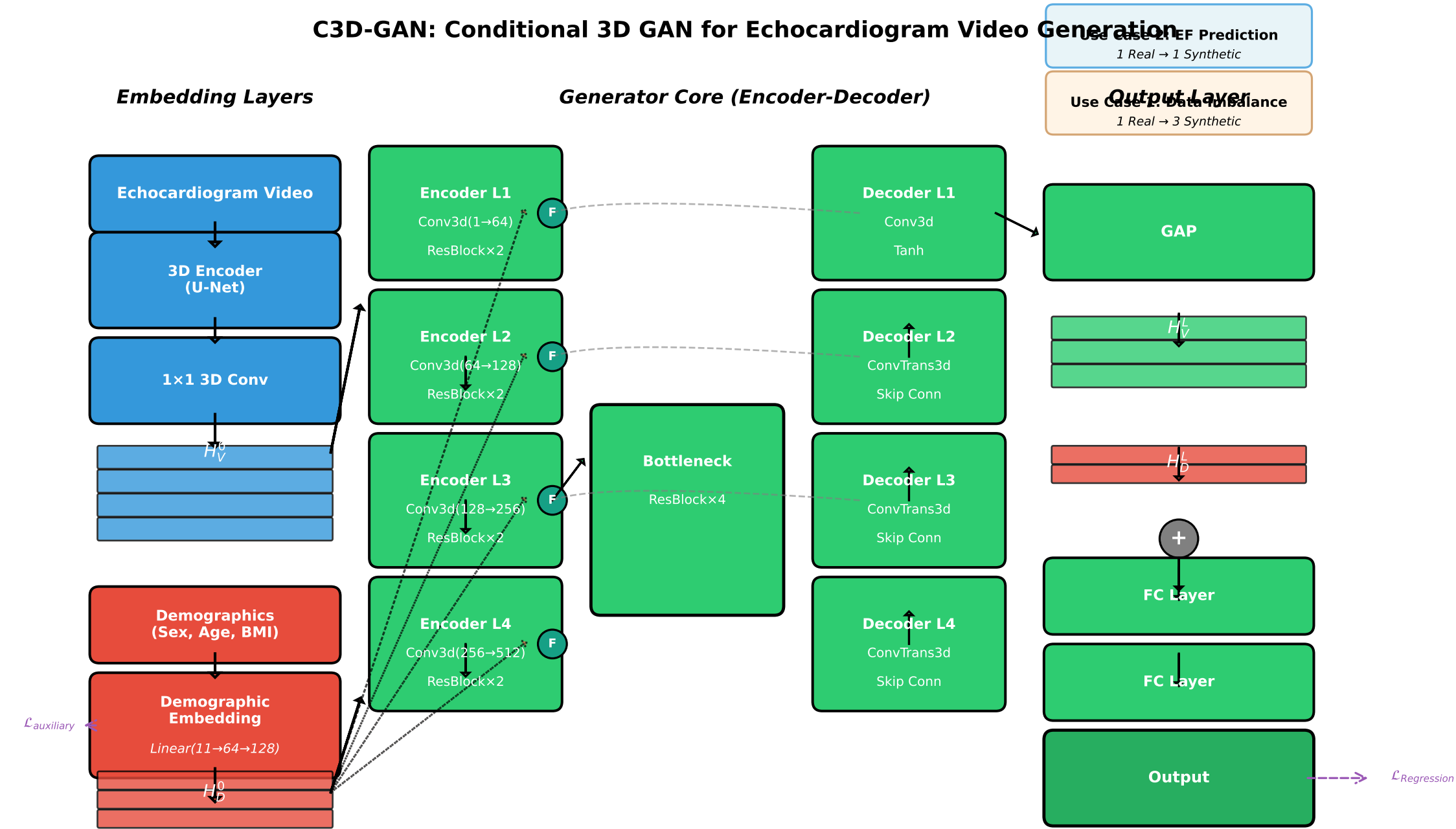
Fig. 1: C3D-GAN consists of: (1) the video embedding layers from echocardiograms, (2) the demographic embedding layers, (3) the generator core with encoder-decoder layers and demographic fusion, and (4) the output layers. The embedding layers extract latent variables of each modality, and the generator core captures their interactions through multi-level demographic fusion. Two use cases: (a) 1 real → 3 synthetic videos for addressing data imbalance, (b) 1 real → 1 synthetic video for EF prediction.
