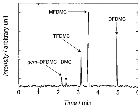
Figure 1. Gas chromatograph of the reaction mixture obtained after the introduction of F_2 gas for 24 hr.
