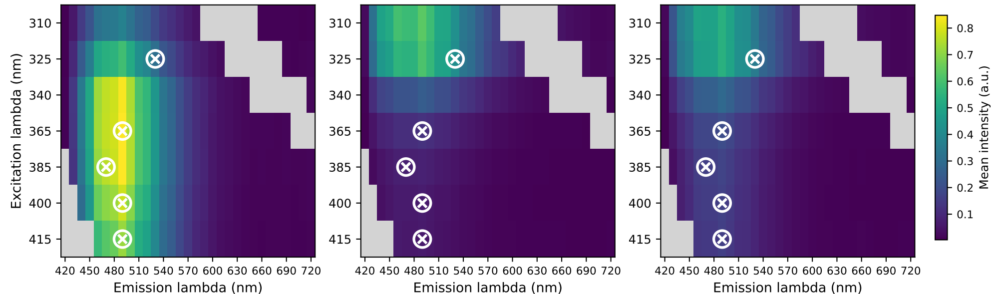
Excitation-Emission Matrix per drop type · K=5 selected (ex, em) shown as circles
