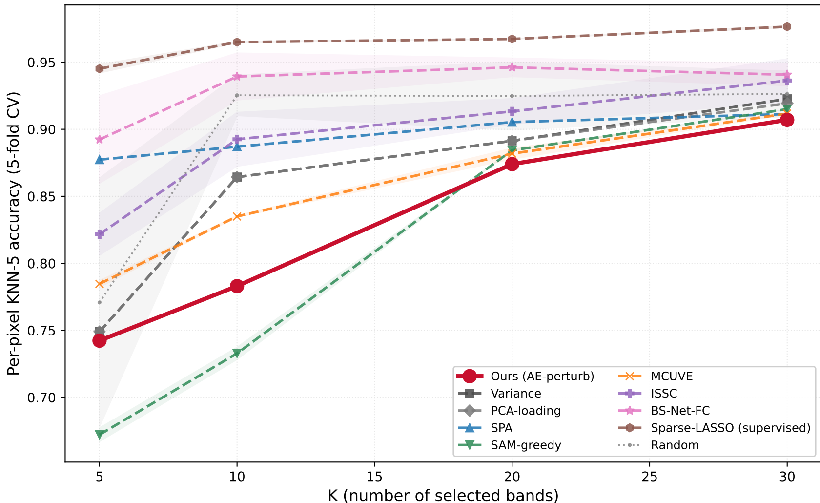
Pepsin-Collagen Dataset: K-band classification accuracy across methods Supervised Sparse-LASSO wins; AE-perturb (ours) is competitive in mid-K range.
