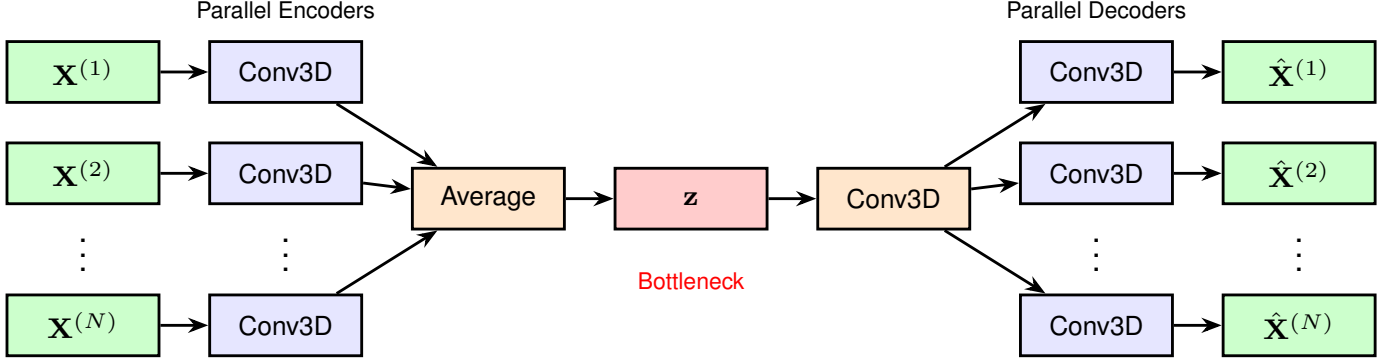
Fig. 2: 3D CAE architecture with parallel branches. Each excitation is processed by a dedicated encoder branch; features are averaged into a shared latent space; parallel decoder branches reconstruct the original 4D structure.
