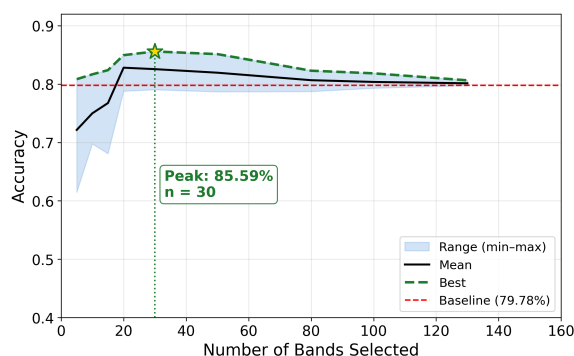
Figure 6: Classification accuracy envelope as a function of band count for the collagen sponge dataset. The best selection exceeds the full-spectrum baseline (79.8%) across a wide range and peaks at 85.6% with 30 of 158 bands. The same pipeline was applied without retuning.
