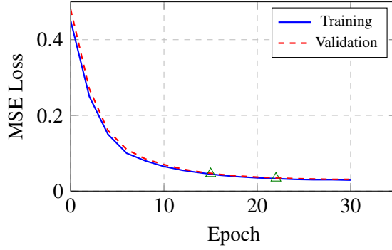
Figure 1: Training convergence curves for the 3D CAE. Loss decreased smoothly from 0.45 to 0.03 over 30 epochs. Green triangles indicate learning rate reductions.
