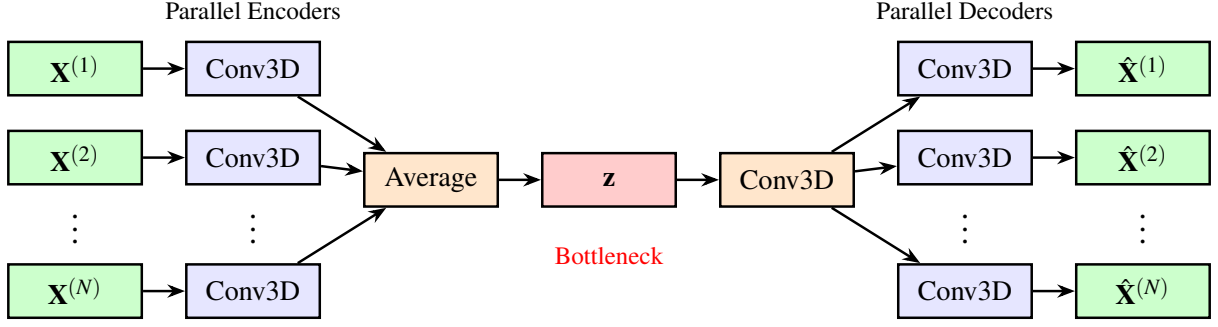
Figure 9: 3D CAE architecture with parallel branches. Each excitation is processed by a dedicated encoder branch; features are averaged into a shared latent space; parallel decoder branches reconstruct the original 4D structure.
