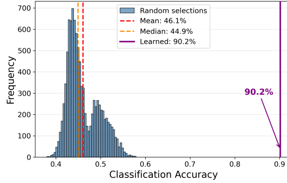
Figure 4: Distribution of classification accuracies for 10,000 randomly sampled 13-band combinations. The histogram shows that random selections cluster around 46% accuracy (dashed lines indicate mean and median), while the learned selection (solid purple line at 90.2%) lies far in the upper tail, outperforming every random combination tested.
