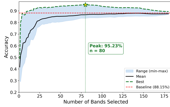
Figure 2: Classification accuracy envelope as a function of band count.
