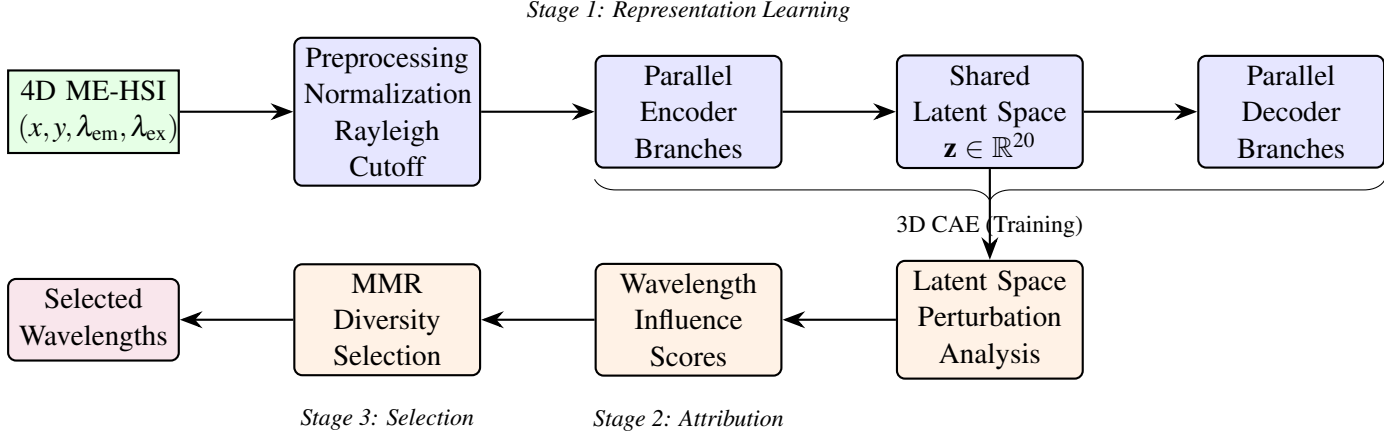
Figure 8: Overview of the proposed wavelength selection framework. The pipeline comprises three stages: (1) a 3D CAE learns a compressed representation of 4D ME-HSI data; (2) perturbation analysis attributes latent dimensions to individual wavelengths; (3) MMR selection identifies diverse, informative band subsets.
