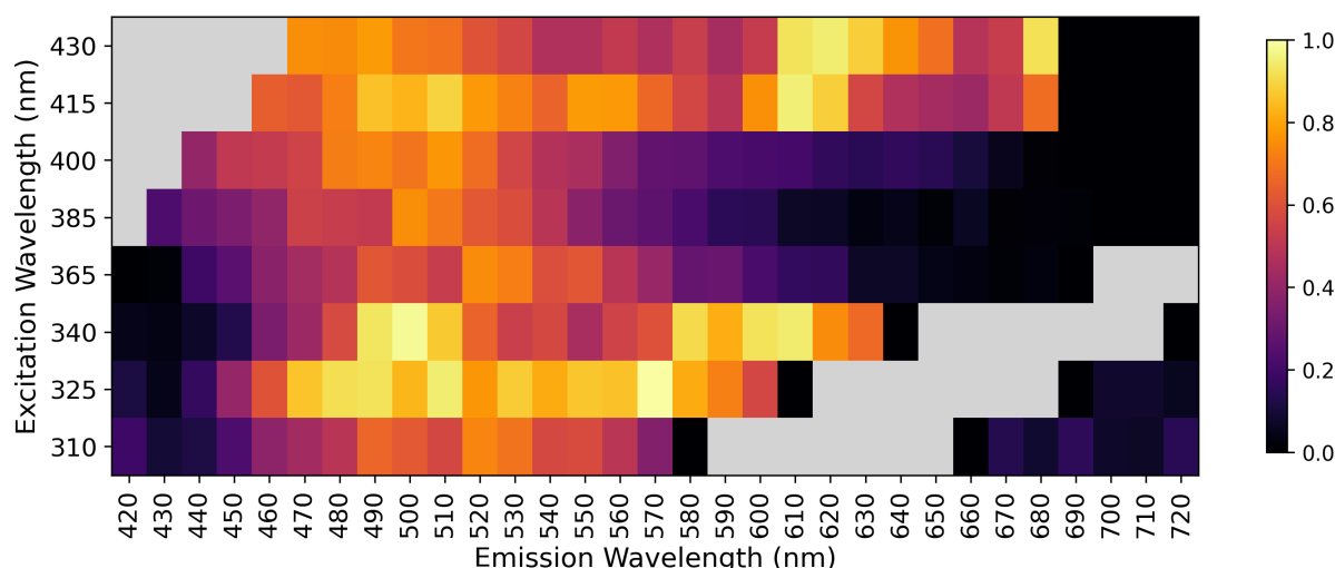
Figure 5: Mean wavelength importance score across the 16 above-baseline configuration groups. Each cell shows the average normalized rank (1.0 = consistently top-ranked, 0.0 = lowest-ranked) for each excitation-emission pair. Grey cells indicate wavelengths excluded by Rayleigh scattering cutoffs.
