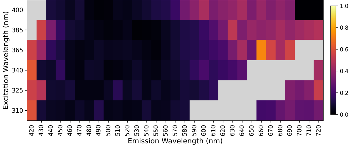
Figure 7: Mean wavelength importance score for the collagen sponge dataset across the above-baseline configuration groups, in the same format as Figure 5. Grey cells indicate wavelengths excluded by Rayleigh scattering cutoffs.
